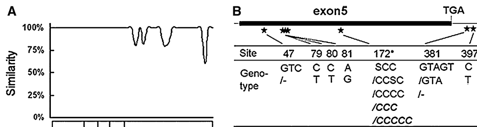
Fig. 5 a Diversity of predicted amino acids in 10 maize inbred lines and eight landraces. The five exons are indicated by open boxes at the bottom. The similarity was averaged over every five aligned amino acids. b Nucleotide diversity in the fifth exon and the 3' UTR of ZmGS3 among 121 maize inbred lines. Site is given according to the position
