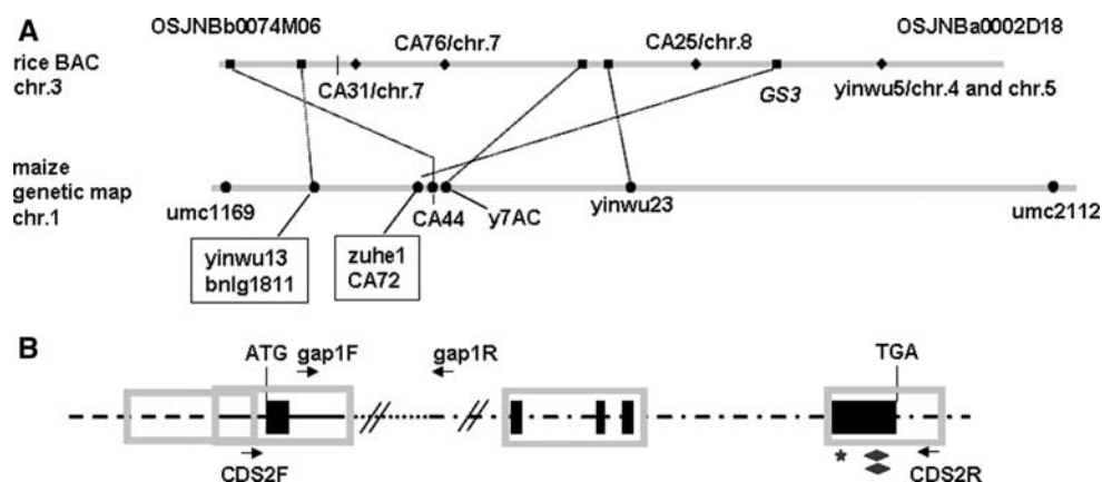
Fig. 1 a Collinear relationship between the rice GS3 region and the corresponding maize region. Squares represent rice genes mapped onto maize chromosome 1. Diamonds indicate rice genes mapped onto other maize chromosomes, with the primers' name and their locations on the maize genetic map being given above or below the diamonds. All rice genes were from two overlapping BAC clones (OSJNBb0074M06 and OSJNBa0002D18). Dots represent maize markers used for genetic mapping, and primers in the open boxes represent co-segregating markers. b Structure of the ZmGS3 gene. Filled boxes represent exons. Black solid line and dash-dotted line represent
